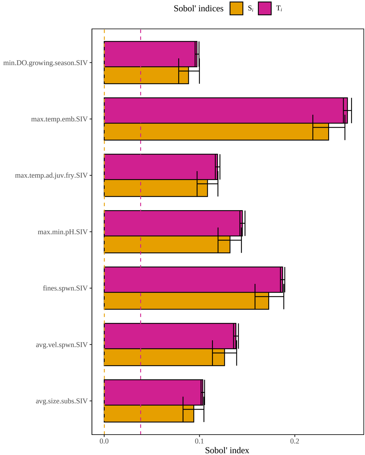
Figure 5. Results of a sensitivity analysis for the brooktroutLacAllLtoe15C model based on a geometric mean structure. Dashed lines represent baseline numerical approximation error for S_i and T_i ( i.e. , dummy variables).
