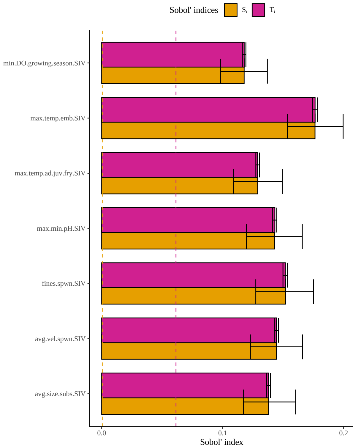
Figure 4. Results of a sensitivity analysis for the brooktroutLacAllLtoe15C model based on an arithmetic mean structure. Dashed lines represent baseline numerical approximation error for S_i and T_i ( i.e. , dummy variables).
